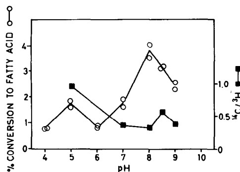
Fig.1. Hydrolysis of alkyldiacylglycerol at different pH. Liver homogenate (1.9 mg protein) was incubated for 15 min with 0.25 mM of each of 1,2- ^3\text{H} dioleoyl-3- O -tetradecyl- sn -glycerol and 1- O -tetradecyl-2,3- ^{14}\text{C} dioleoyl- sn -glycerol solubilized in lecithin and albumin as described under Materials and methods. Open symbols show the conversion of the ^3\text{H} -substrate to fatty acid and the black symbols show the ^{14}\text{C}/^3\text{H} ratio in fatty acid (ratio in substrate = 1.00).
