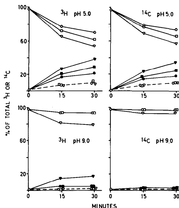
Fig.2. Effect of albumin and Triton X-100 on alkyldiacylglycerol hydrolysis at pH 5.0 and pH 9.0. Liver homogenate was incubated with the racemic substrate described in fig.1, although the basal incubation (○ ●) did not contain albumin. 1.6% Albumin (▼ ▼) or 0.08% Triton X-100 (□ □) were added where indicated and the final incubation mixture was sonicated for 10 s. The amount of radioactivity in alkyldiacylglycerol (○—○, ▼—▼, □—□) alkylmonoacylglycerol (○--○, ▼--▼, □--□) and fatty acid (●—●, ▼—▼, ■—■) is shown.
